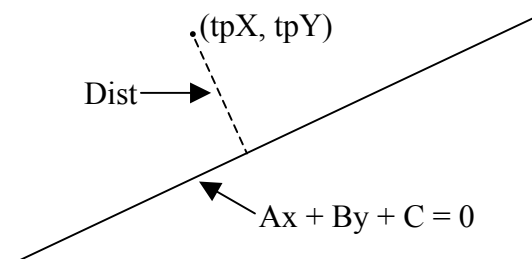
Fig. CS1-2 Distance from a point to a line
