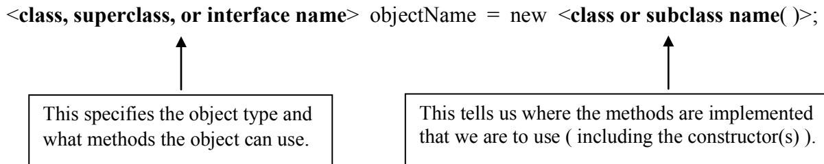
Fig. 38-1 Determining object type, legal methods, and where the methods are implemented. If a method in the subclass overrides that of the superclass, then code in the subclass runs.
